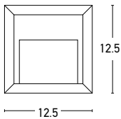
E 130 D: 12.5x12.5x2.5 ≡ 1.5W LED 3000K, IP65 Material: Plastic Available Color: Grey
