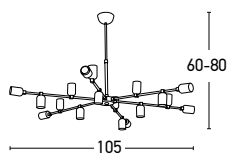
1485 18L D: Ø105 H60-80 18x E27 MAX 40W Material: Steel Available Color: Copper Rusty
