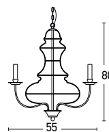
17116 D: Ø55 H80 3xE14 MAX 40W Available Chain: 50 cm
