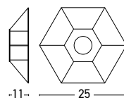
1556 D: Ø25 H11 E14 MAX 40W Material: Steel Available Color: Copper Rusty
