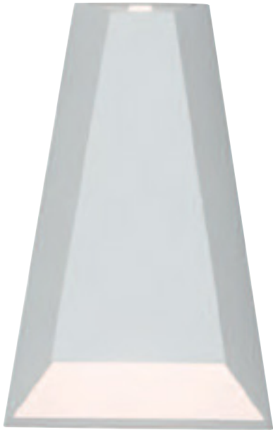
E 156 D: 6.5 H17.5 L11 2x3W LED 3000K Cree, IP54 Material: Aluminium-Glass Diffuser Available Color: White
