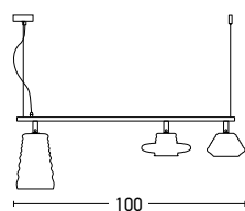
1431 3L D: Ø100x20 3x E27 MAX 40W Material: Glass Available Color: Chrome-Black Available Cable: 100 cm
