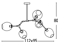
1696 D: 112x95 H80 5x E27 MAX 40W Material: Metal-Glass Available Color: Black
