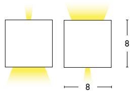
E 109 D: 8x8x8.2 2x3W LED 3000K Cree, IP54 Material: Aluminium-Glass Diffuser Available Color: Graphite
